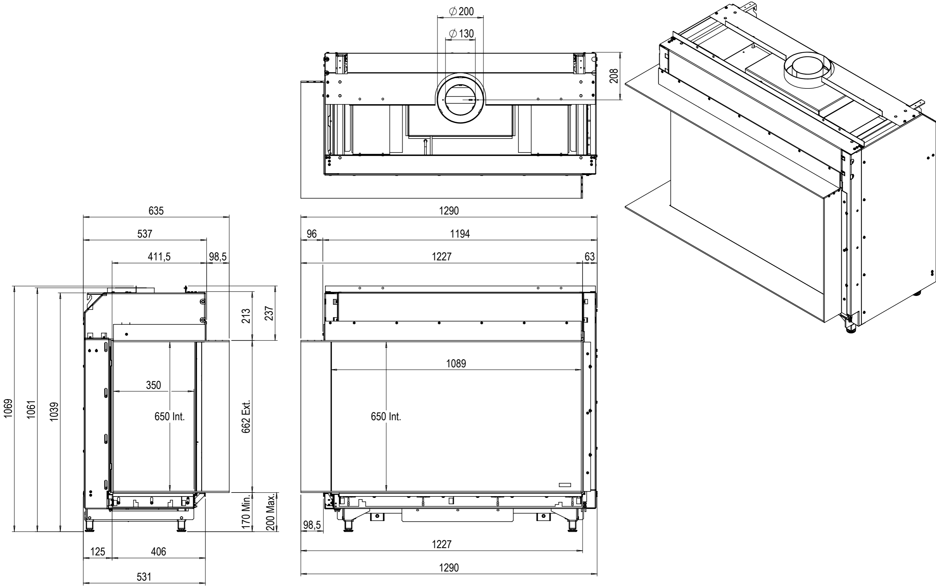
Dimension drawing 1050-650 - II (100)
