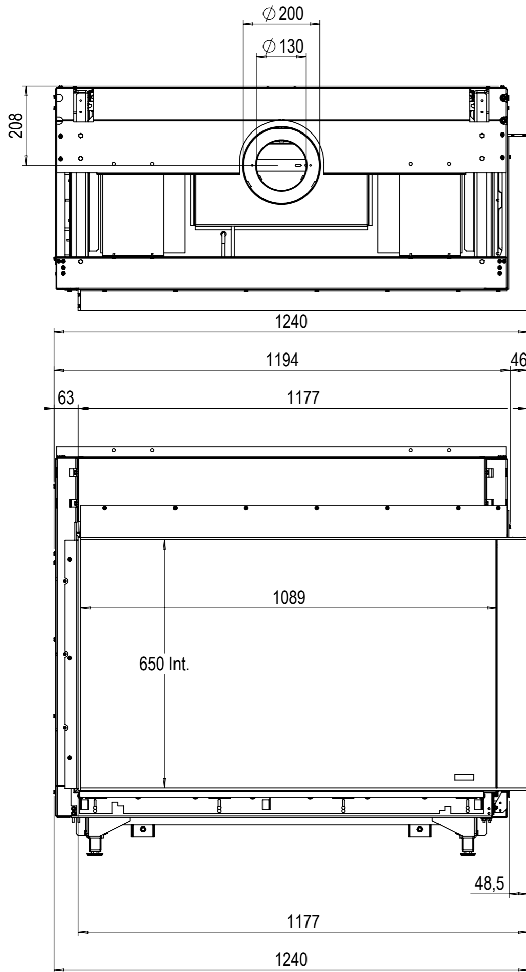
Dimensional drawing 1050-650 - II R (50)
